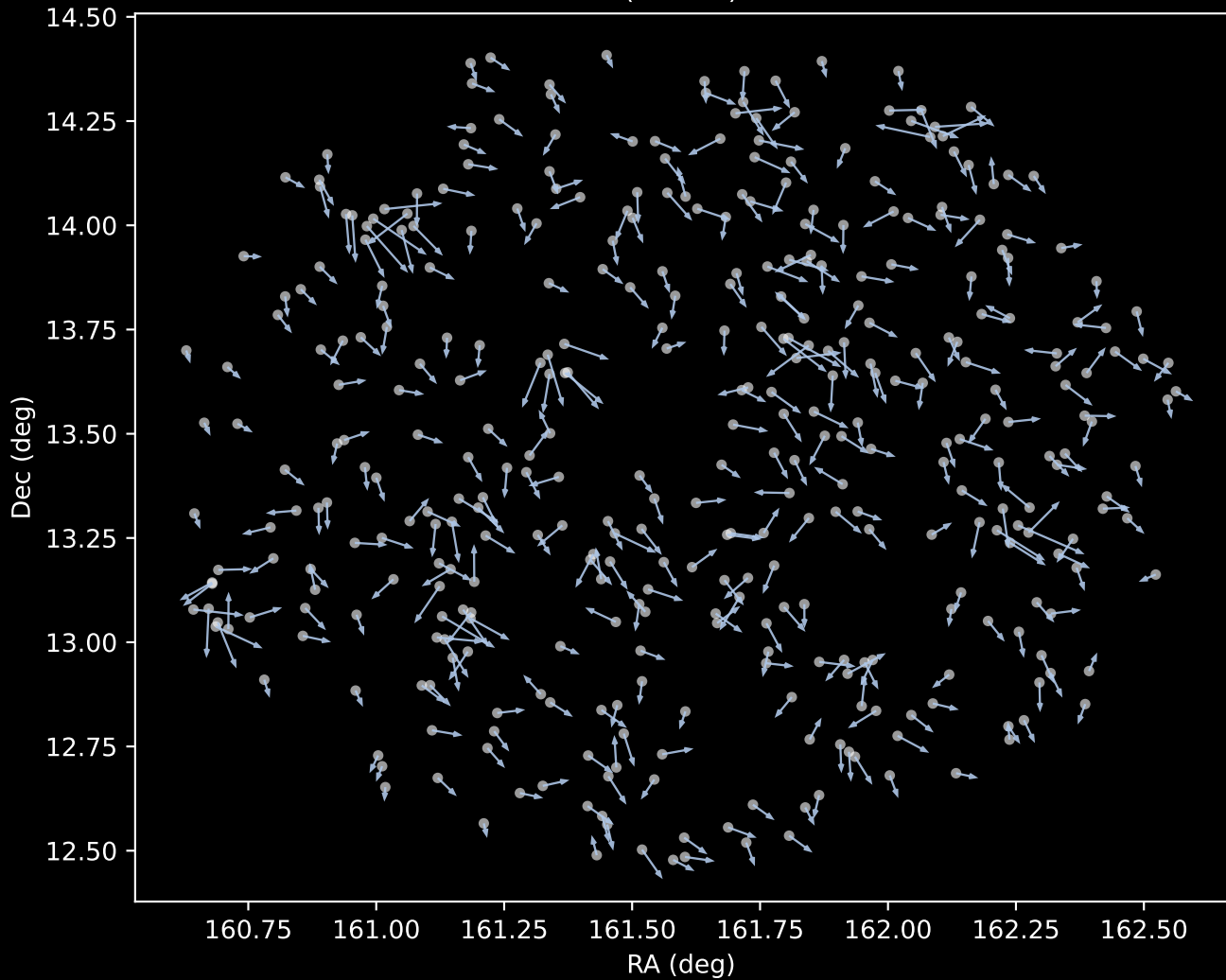
GALAH DR4 Cluster 1 Proper Motion Vectors (n=378)
