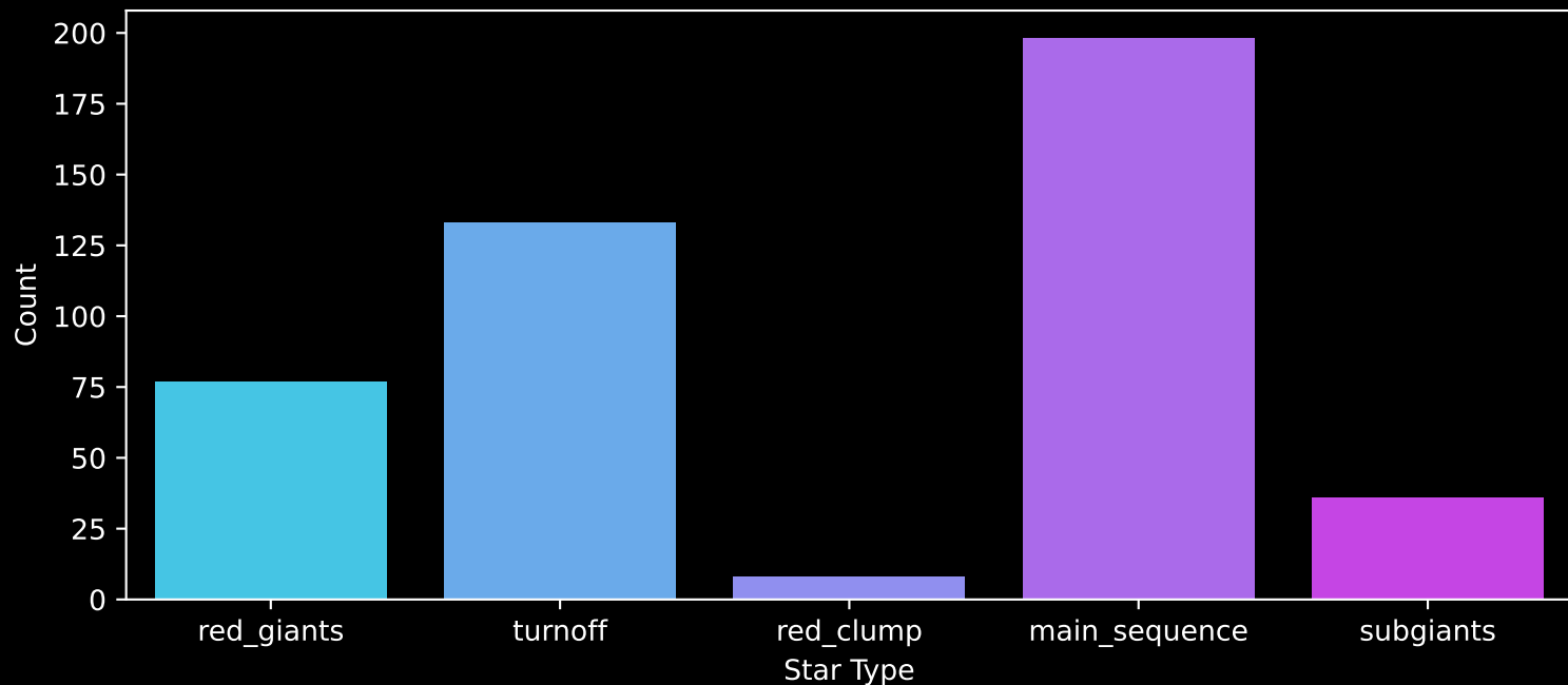
GALAH DR4 Field: [6590] Count plot of Star Type
