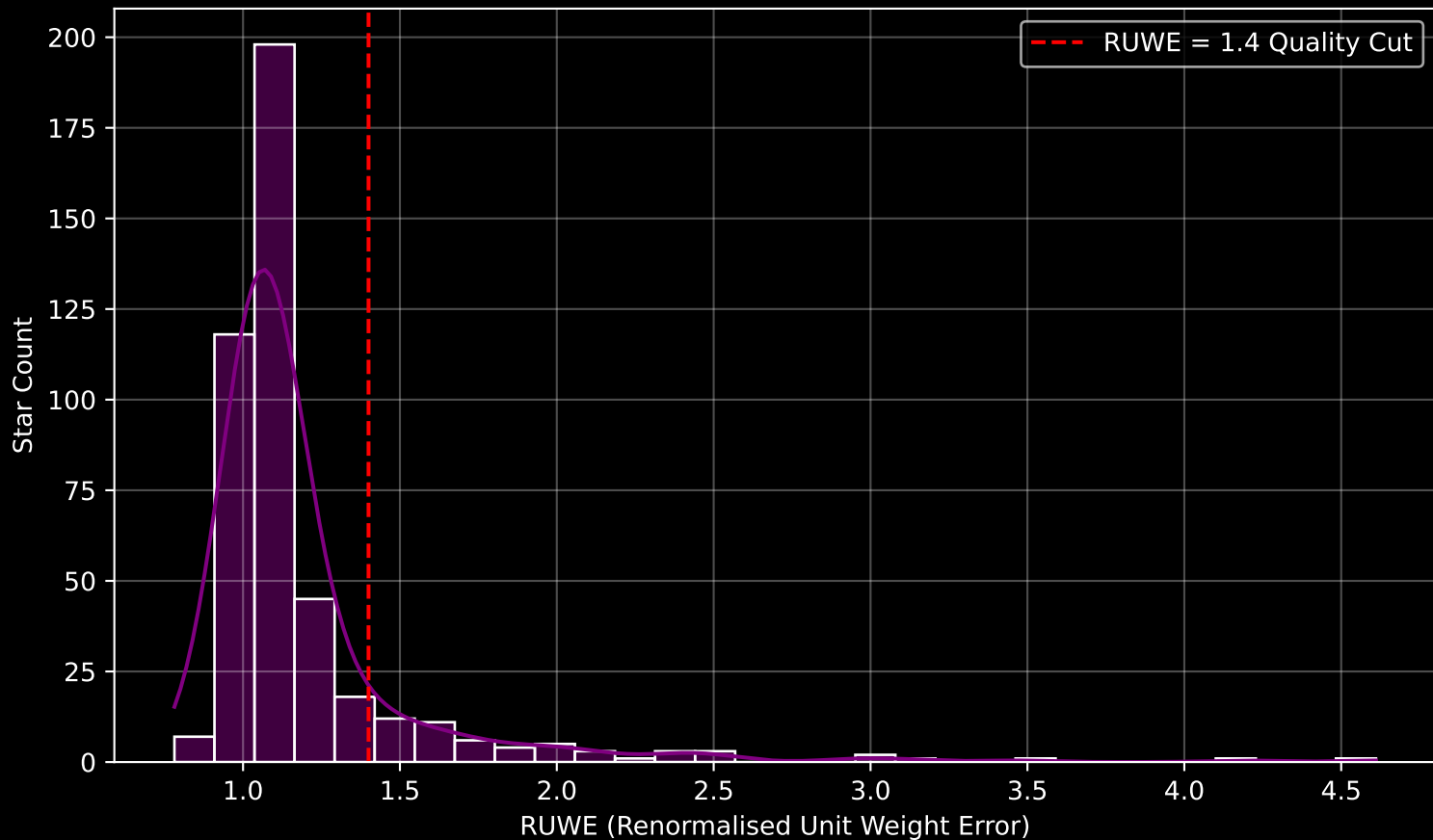
GALAH DR4 Field [6590] RUWE Distribution (n= 440)
