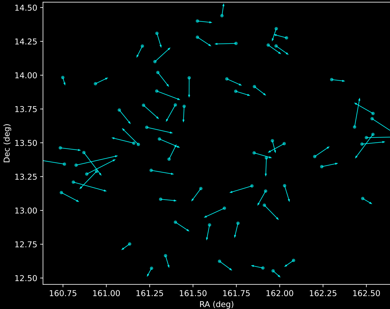
GALAH DR4 Noise Stream Proper Motion Vectors (n=68)
